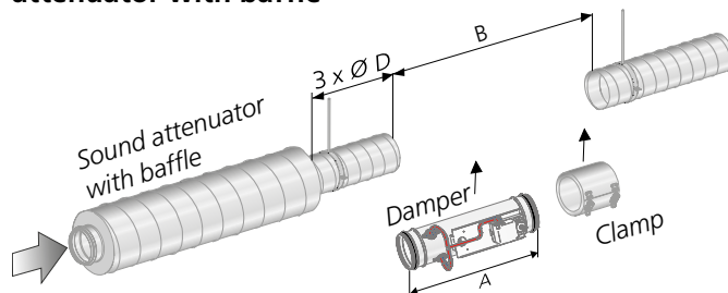
Figure 5. Straight duct section requirements 3 x Ø in case of sound attenuator with baffle or centre body.
