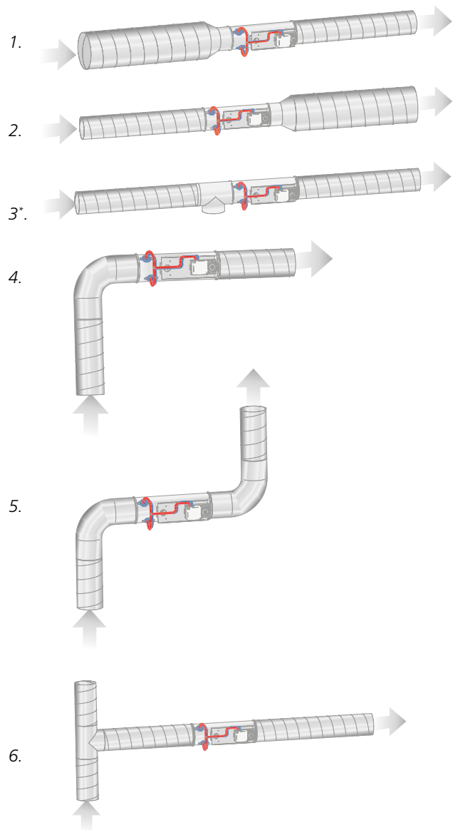
Figure 4. Straight duct section requirements in circular ducts, number of Ø before product: Image 1-5 require no straight duct section (image 3* illustrates a T piece with a cleaning hatch). Image 6 requires a straight duct section before the damper equivalent to 4 x the diameter of the duct.
