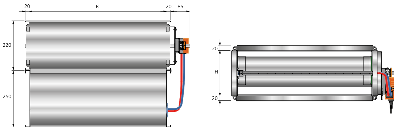
Figure 7. Dimensions (mm), REACT V BBAC rectangular.
