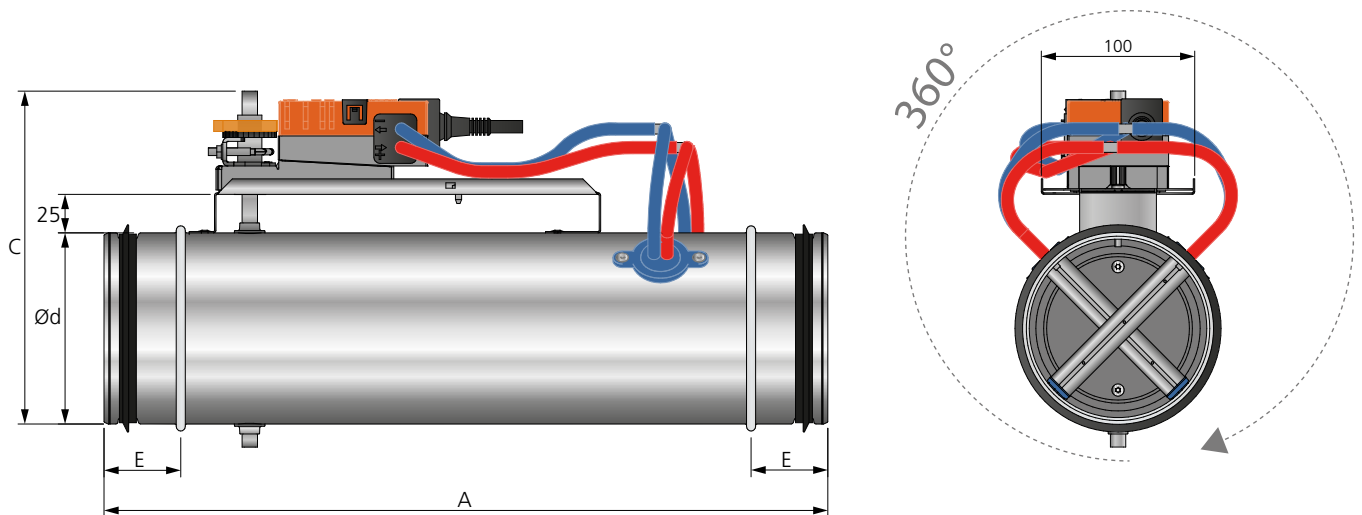
Figure 3. Dimensions (mm), REACT V BBAC circular. The damper can be installed at an optional angle.
