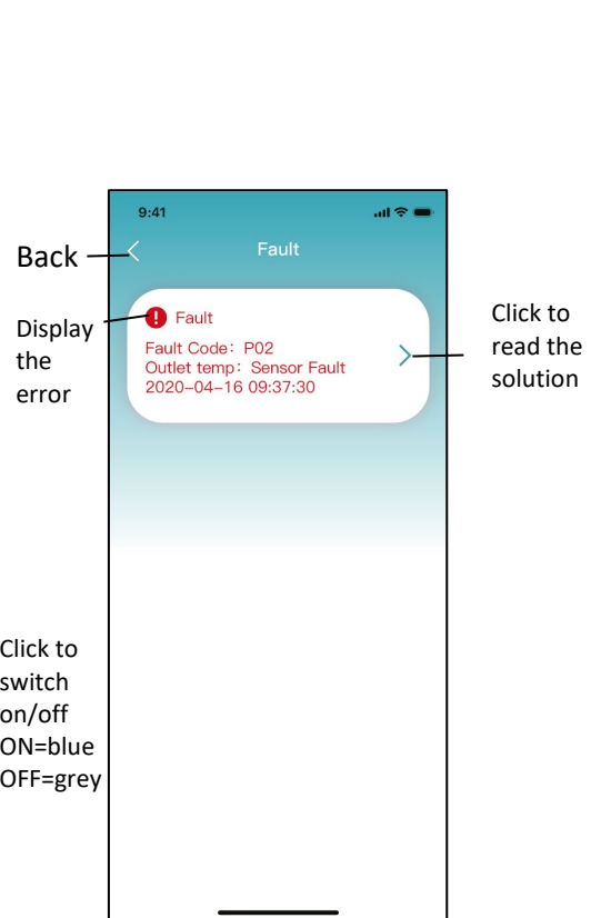
Fig.24 Troubleshooting interface
