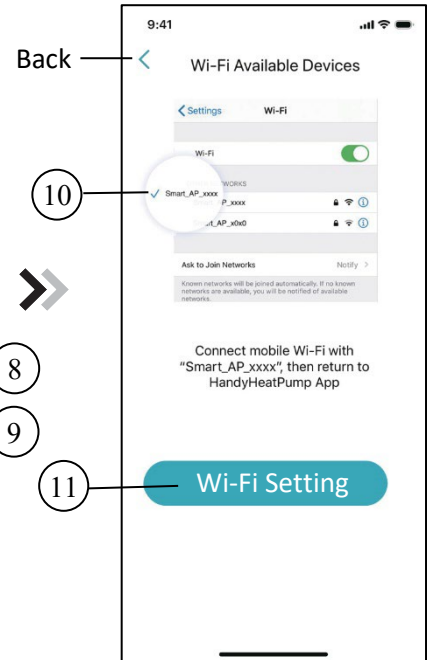
Fig.9 Connect specified
